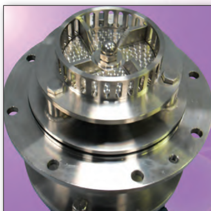
Bottom entry high shear option
